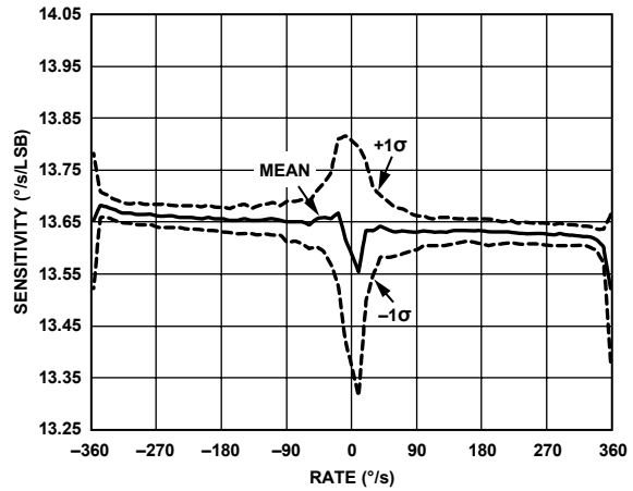
Figure 20. Gyroscope Linearity
